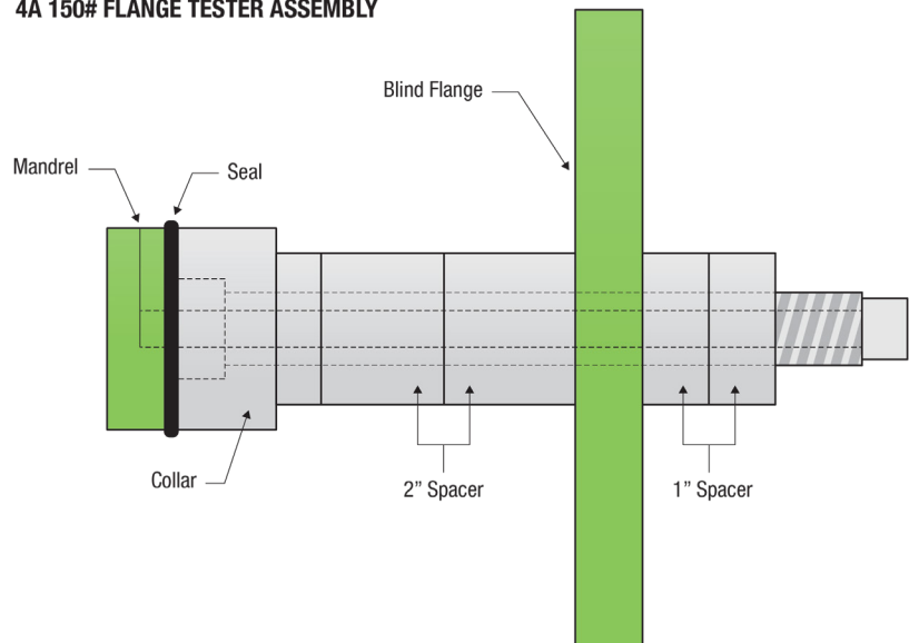
4A 150# FLANGE TESTER ASSEMBLY
